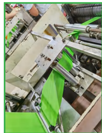
折膜 Split film
